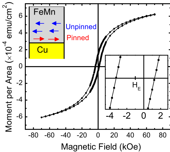
FIG. 1. Magnetic hysteresis loop of the Ta(5-nm)/[Cu(5-nm)/FeMn(5-nm)] 10 /Ta(5-nm) stack measured at 10 K after a 70-kOe-magnetic-field cooling. The bottom-right inset shows the central part of the loop with a clear indication of exchange bias shift. The exchange bias field is H_E = -985 Oe. The top-left inset depicts the pinned and unpinned uncompensated magnetic moments inside the FeMn layer; the compensated antiferromagnetic spin structure is not shown.
