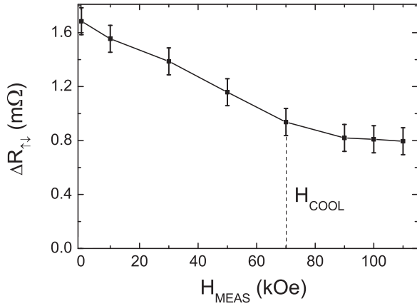
FIG. 3. The difference in resistances measured at 180^\circ and 0^\circ , \Delta R_{\uparrow\downarrow} at T = 10 K after field cooling at \Theta_{COOL} = 0^\circ for the Ta(5-nm)/Cu(5-nm)/Py(2-nm)/Cu(5-nm)/FeMn(5-nm)/Cu(5-nm)/Ta(5-nm) AFSV as a function of magnetic-field H_{MEAS} applied during the measurement.
