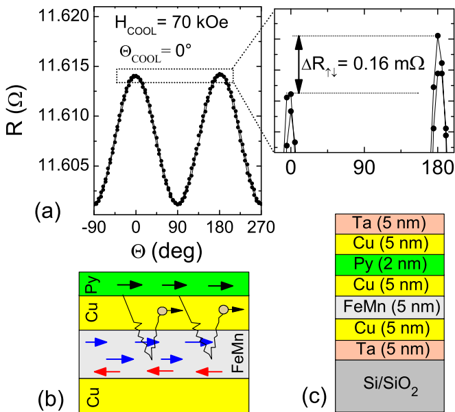
FIG. 4. (a) Angular dependence of the resistance of the Ta(5-nm)/Cu(5-nm)/FeMn(5-nm)/Cu(5-nm)/Py(2-nm)/Cu(5-nm)/Ta(5-nm) AFSV measured in 70 kOe after the AFSV was cooled down in H_{\text{COOL}} = 70 kOe applied at \Theta_{\text{COOL}} = 0^\circ . The inset in the top-right corner shows the magnified peaks. (b) and (c) are schematics illustrating the scattering of polarized electrons at the Cu/FeMn interface and the structure of the AFSV, respectively.
