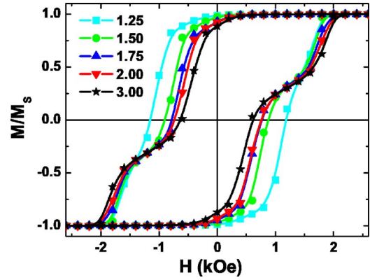
FIG. 1. (Color online) Hysteresis loops of two interacting magnetic dots with D=65 \text{ nm} and H=20 \text{ nm} . Squares illustrate the results for two dots with a center-to-center distance d=1.25D , circles corresponds to d=1.5D , up triangles correspond to d=1.75D , down triangles correspond to d=2D , and stars to d=3D , which coincides with the case of noninteracting dots. Lines are guide to the eye.
